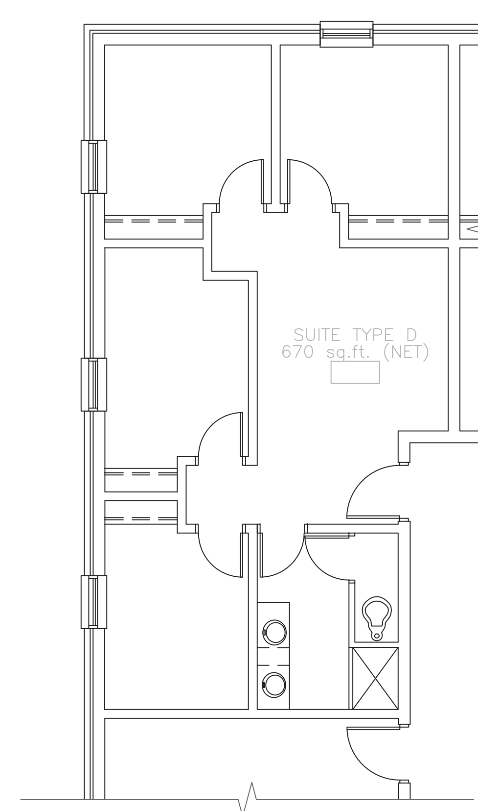
SUITE TYPE D SCALE: 3/16" = 1'-0"
