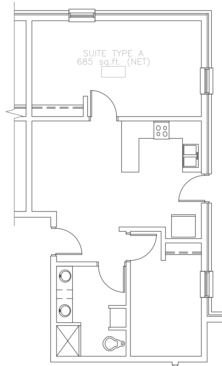
SUITE TYPE A SCALE: 3/16" = 1'-0"
